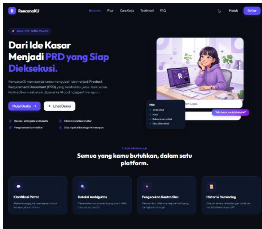
Gambar 1. Home Page.
